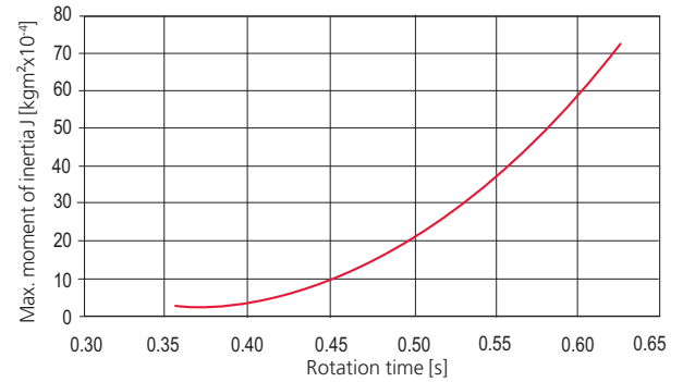
Rotation time RE-50 18-100V, 180° - horizontal with SE-24
