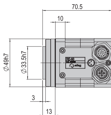
RE-50/ RE-50 18-100V without flange
