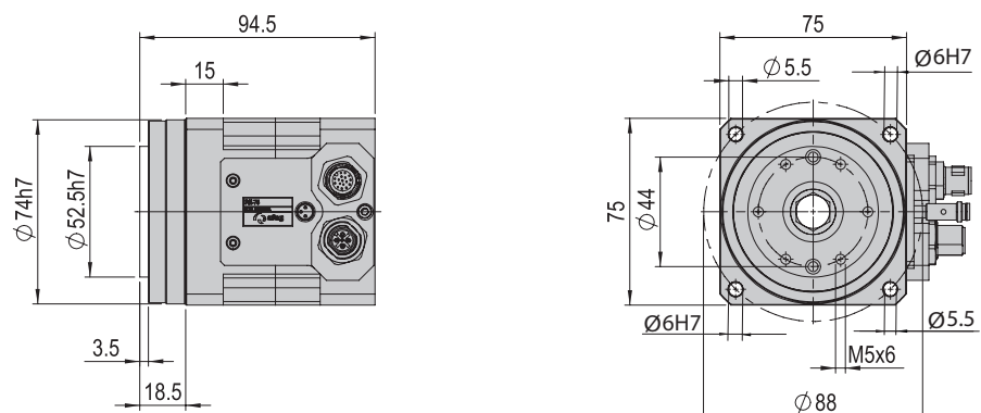
RE-75/ RE-75 18-100V A without flange
