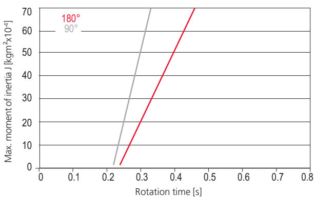
Rotation time
