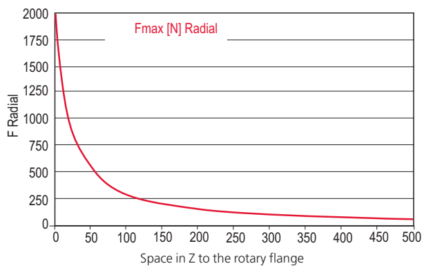
Radial dynamic
