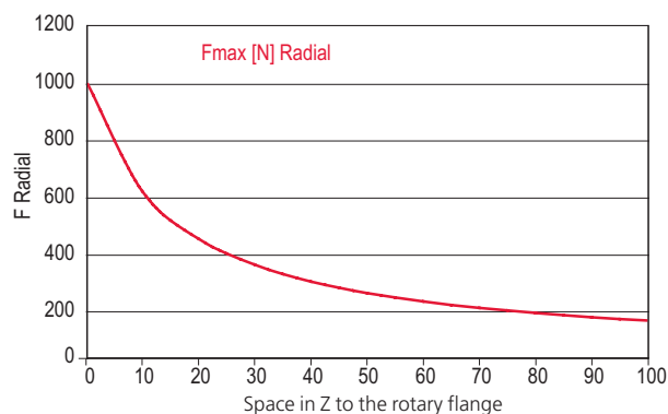
Radial static
