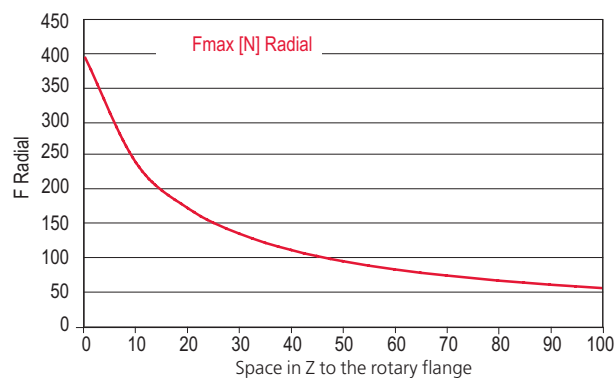
Radial dynamic
