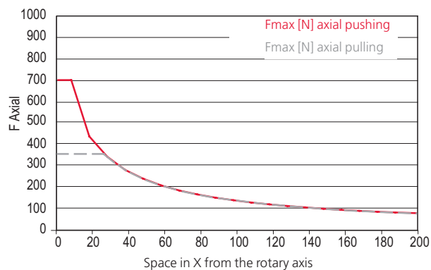
Axial static
