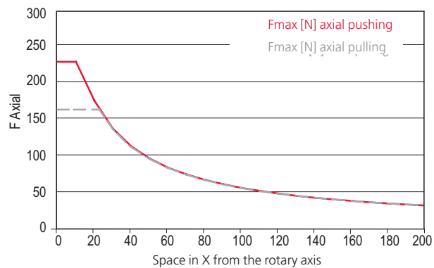
Axial dynamic
